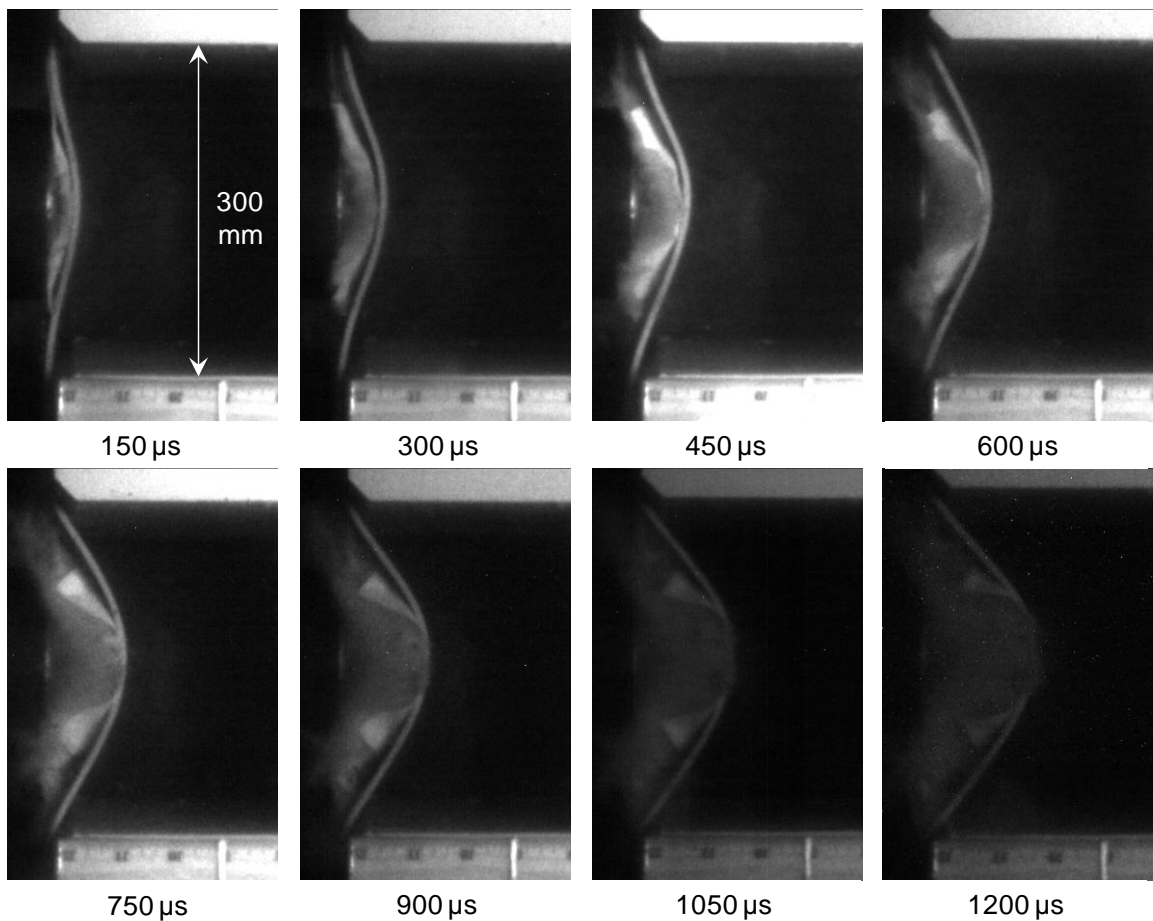
Figure 5.3 Sequence of high-speed photographs showing the deformation in a monolithic composite plate subjected to underwater impulsive loading with \bar{I} = 0.035 .
