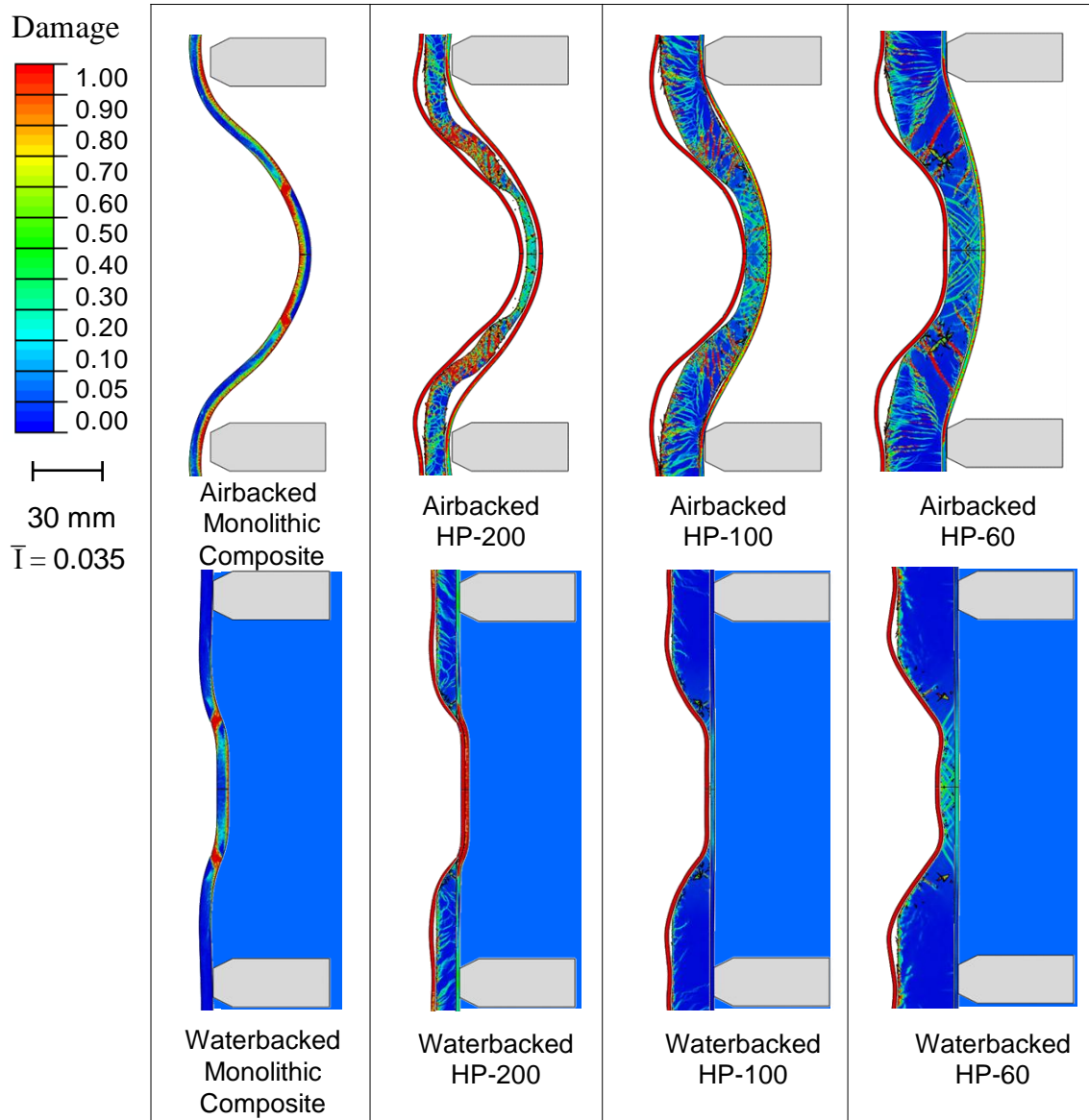
Figure 6.4 Comparison of damage contour plots for different composite structures subjected to underwater impulsive loads under air-backed and water-backed conditions (at t = 1000 \mu\text{s} ). The monolithic structure transmits the impulse instantaneously. As the core thickness increases , the magnitude and duration of transmitted impulse decreases .
