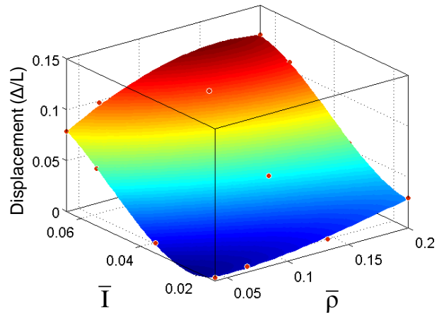
Figure 6.8 Normalized displacement in water-backed structures as a function of incident impulse \bar{I} and core relative density \bar{\rho} .
