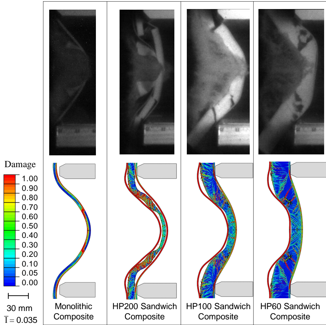
Figure 5.11 Comparison of experimental and computational deformation sequences for different composite structures at 1000 \mu\text{s} . The dynamic deformations and failure modes are accurately captured in the finite element simulations including matrix-cracking, core-cracking, core-face debonding and core-crushing. Note that rate-effects are not implemented in the simulations.
