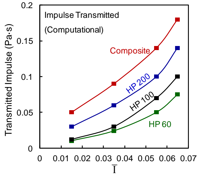
Figure 5.14 Computational results for transmitted impulses as a function of peak-pressure for different composite structures.
