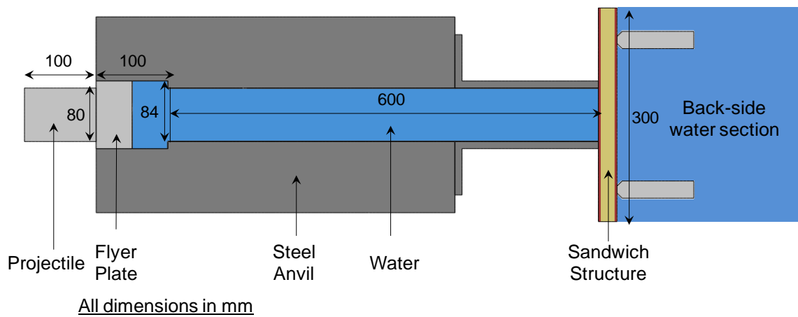
Figure 6.2 Sectional view of a simply-supported sandwich structure in water-backed conditions.
