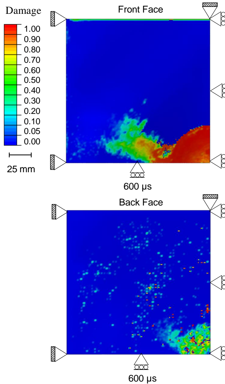
Figure 7.5 Distributions of tensile damage in the matrix of the facesheets at t = 600 \mu\text{s} . T_f/T_c = 0.05 and \bar{I} = 0.2 . The plies shown are oriented horizontally.
