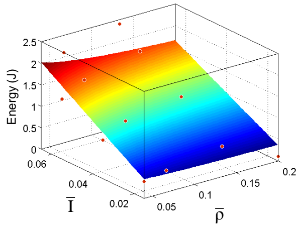
Figure 6.9 Energy dissipated due to inelastic deformation in water-backed structures as a function of incident impulse \bar{I} and core relative density \bar{\rho} .
