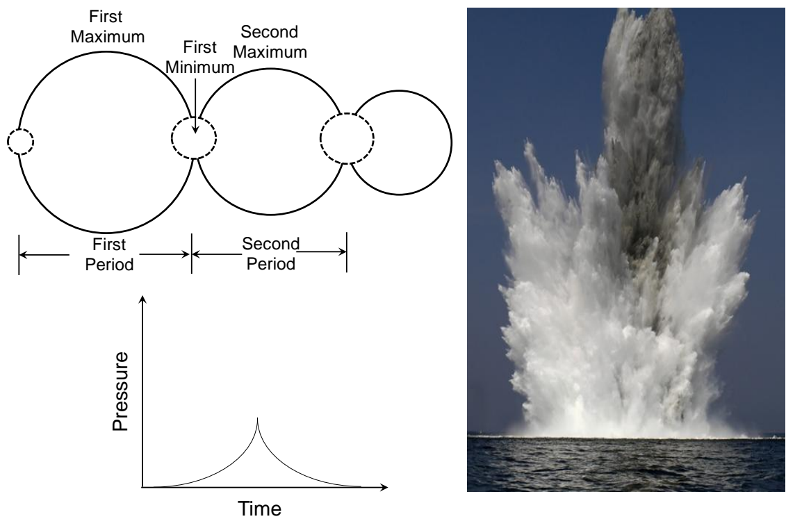
Figure 2.2 Bubble oscillations and pressure profile generated due to oscillations [1] and a "plume" created when an underwater explosion bubble reaches the water surface.
