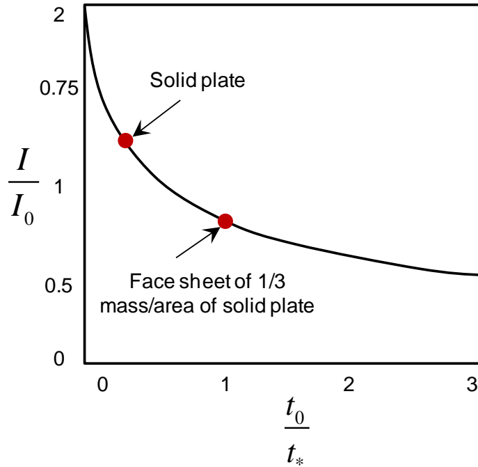
Figure 2.6 Fluid-structure interaction in water: sandwich plate vs. monolithic plate [3, 5].
